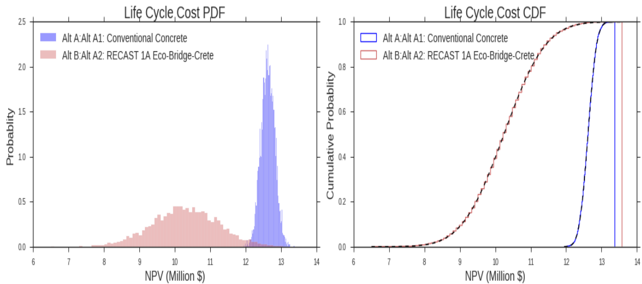
Figure A.9 Bridge LCCA example – probabilistic approach
