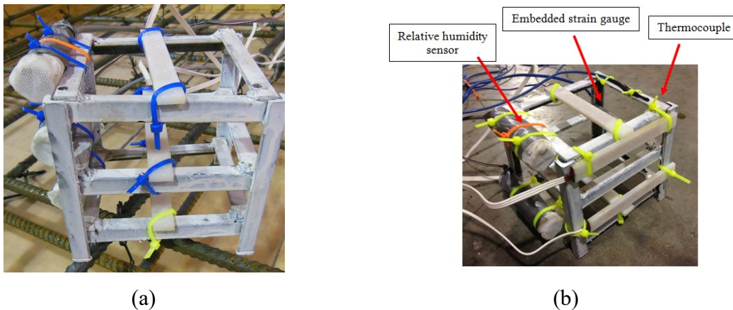
Figure 3.4. Instrumentation layouts for (a) Layout A: 3 embedded strain gauges in longitudinal direction, 3 thermocouples and RH sensors and (b) Layout B: 4 embedded strain gauges (2 longitudinal and 2 transverse directions), 2 thermocouples and 2 RH sensors
