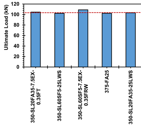
(b) Ultimate load magnitude
