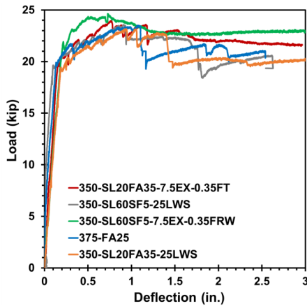
(a) Load-deflection response
