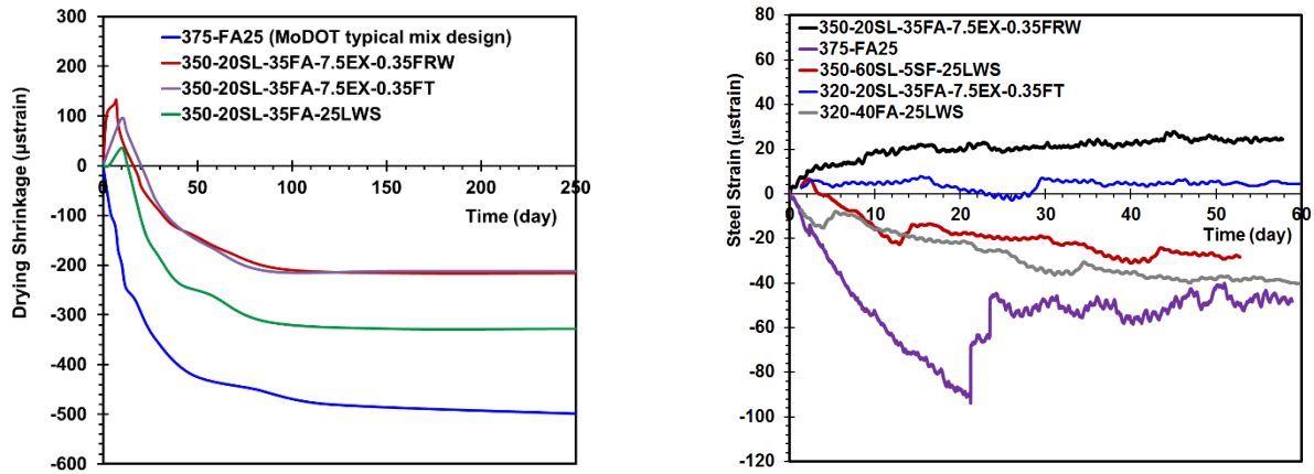
(a) Drying shrinkage
