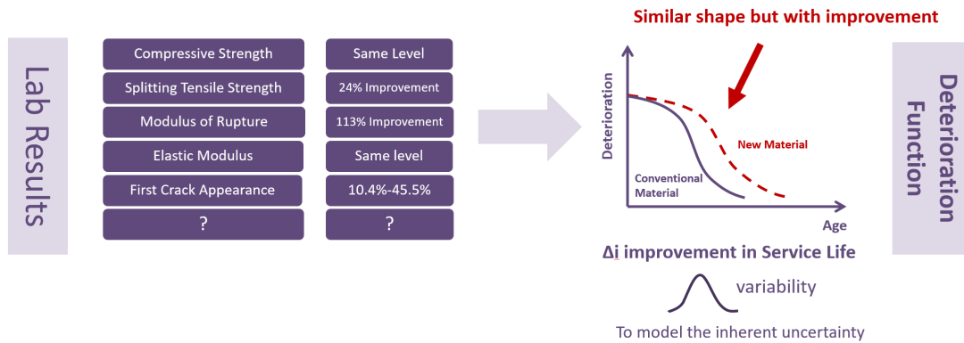
Figure A.5 Using laboratory results to update a deterministic deterioration function
