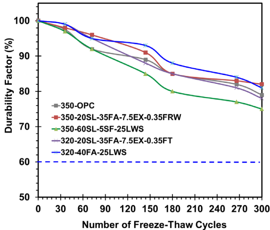
(c) Frost durability factor
