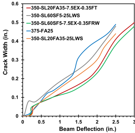
(c) Deflection-crack width relationship
