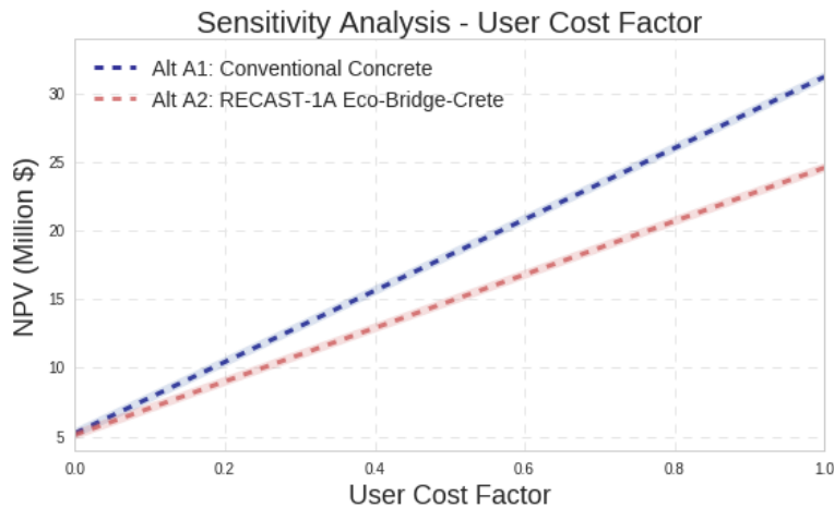
Figure A.8 Sensitivity analysis example (Estimated weight of user cost)
